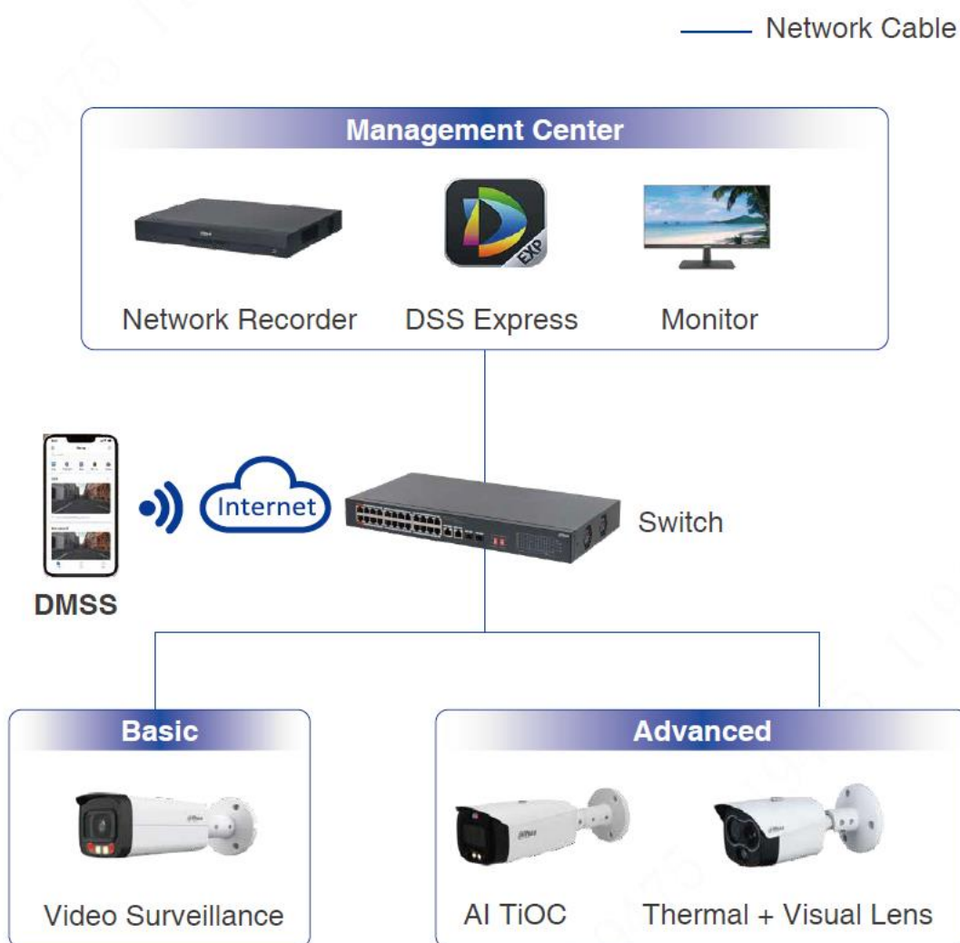
Dahua's AI Perimeter Protection Solution Topology
