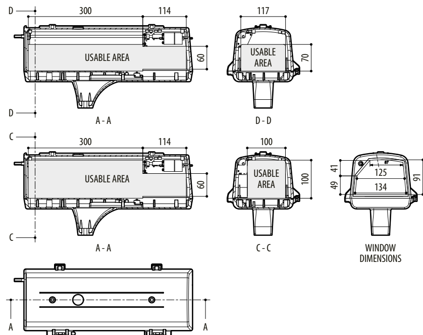
ULISSE2, HOUSING
