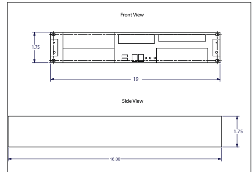
Rack-Mount
