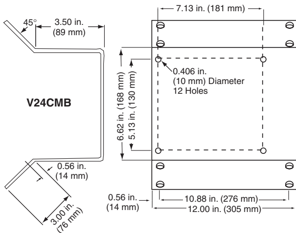
Figure 1: V24CMB/V24CMB-SS Corner Mounting Bracket
