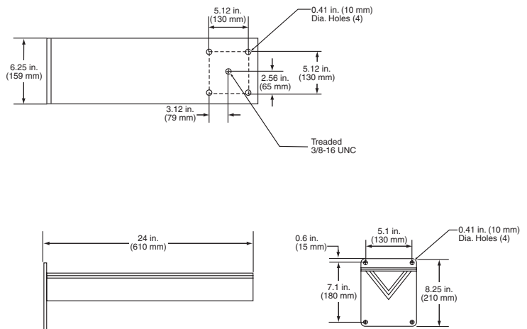
Figure 2: V24WM/V24WM-SS Outline Drawing
