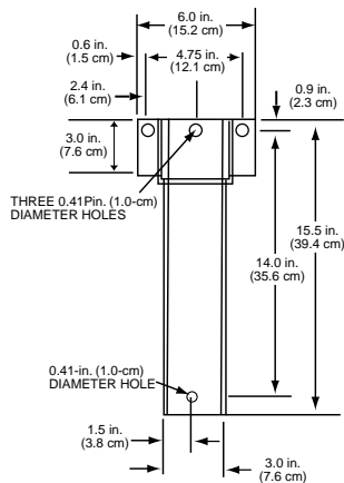
Figure 1 V1502CA Ceiling Mounting Adapter and V1501WM Wall Mounting Adapter
