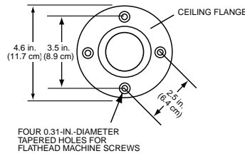
V1502CA CEILING MOUNTING ADAPTER
