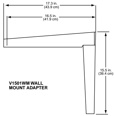
Figure 1 V1502CA Ceiling Mounting Adapter and V1501WM Wall Mounting Adapter
