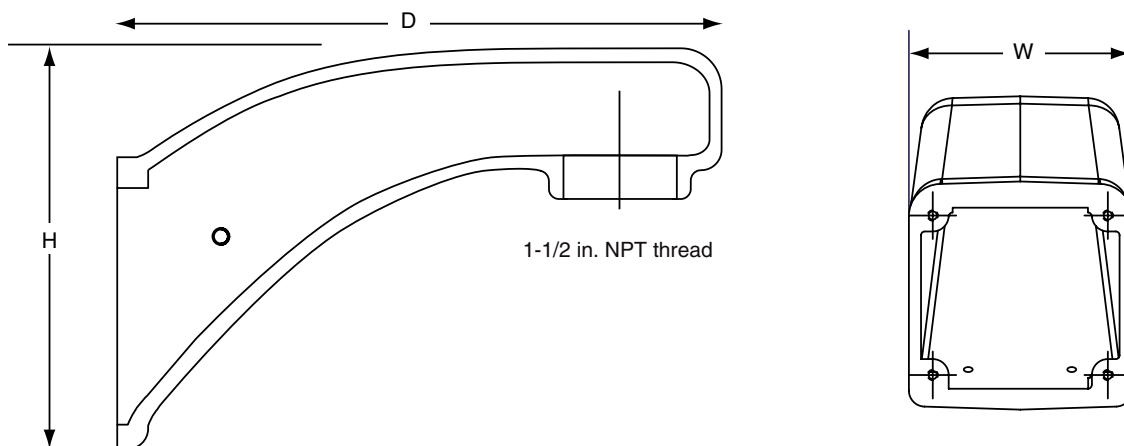
Figure 1: Dimension Drawing
