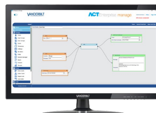
Rules Engine
