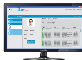
ACT Monitor
