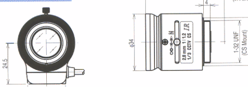
Fixed-Focal Lenses Auto Iris
