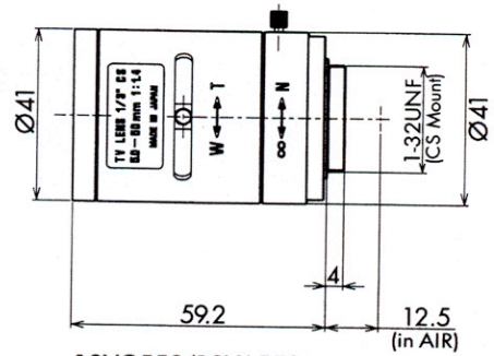
13VG550/13VA550 1/3" 5-50mm 1:1.4 CS Mount DC Iris / Video Iris
