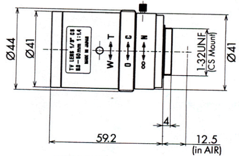
13VM550 1/3" 5-50mm 1:1.4 CS Mount Manual Iris
