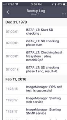
Bootup Log
