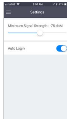
System Settings
