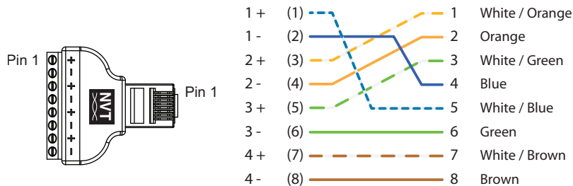
Screw terminal block channel pinout
