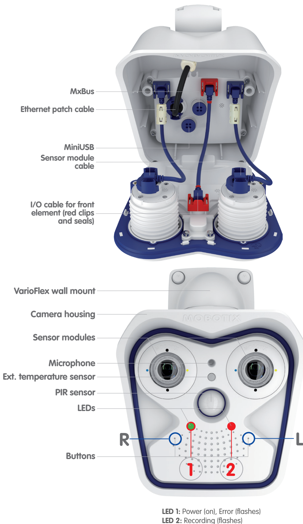
(M15D – Camera housing and connectors, excerpt from the technical documentation)
