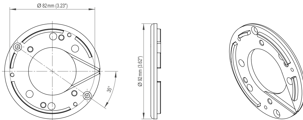
Mounting ring for surface mount variant (compatible with flush-mounted sockets according to DIN 49073)
