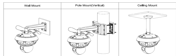
DH-PFA153-SG Pole-mounted bracket
