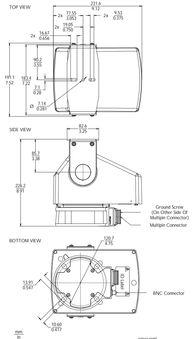
Dimensional Outline
