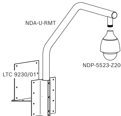
Fig. 4: Roof mount (IP66)
