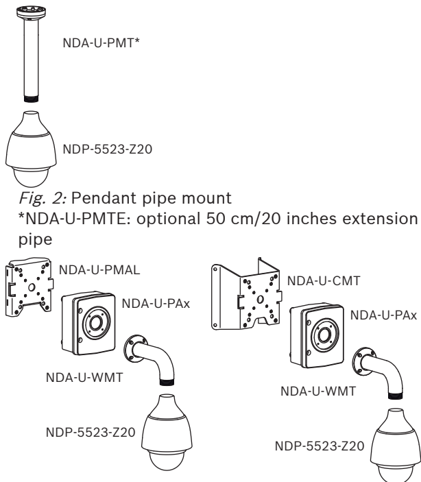
Fig. 3: Pole mount (IP66); Corner mount (IP66)
