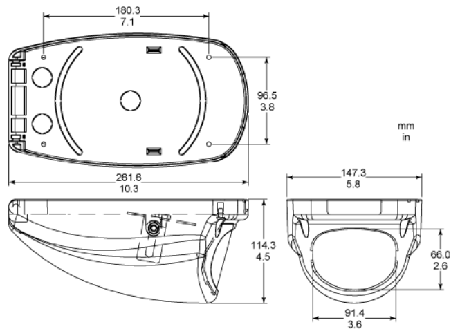
Dimensional Outline
