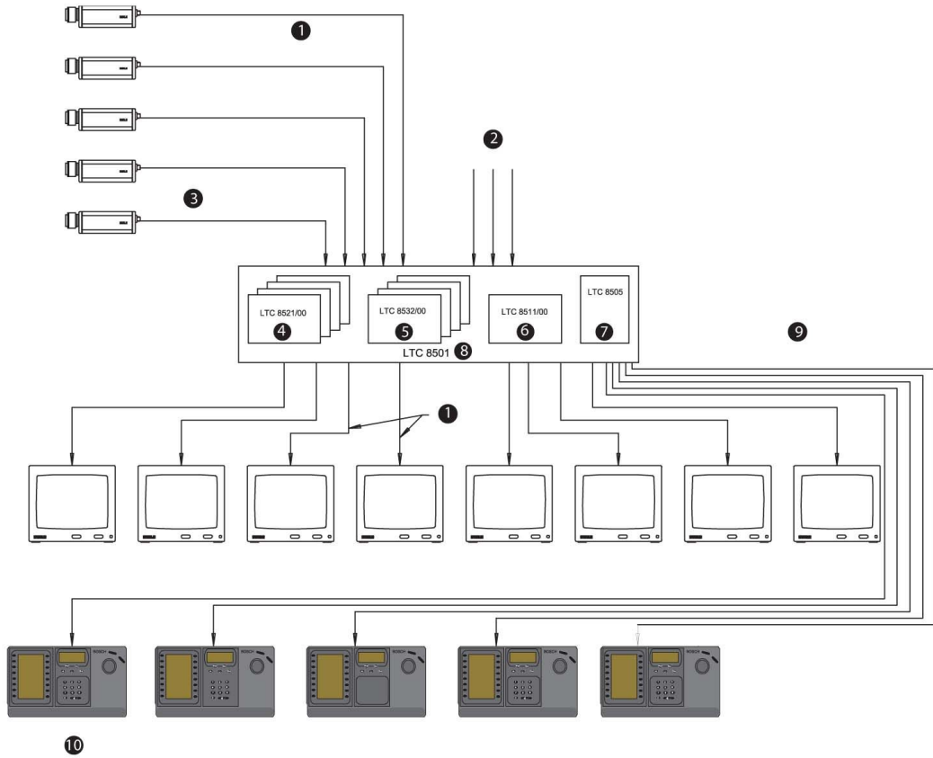
LTC 8500 Series Configuration Diagram (64 Cameras by 8 Monitors)
