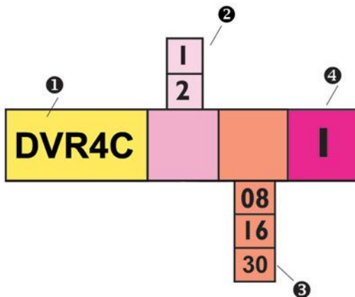
DVR4C Typenumber
