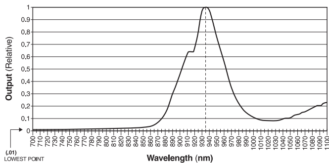
AD1020-6051 Output Characteristics
