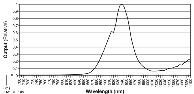
AD1020-1541 Output Characteristics
